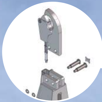
PNEUMATIC HOOK
